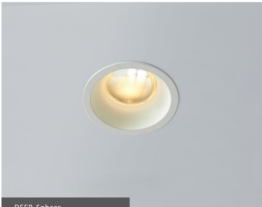
DEEP Sphere
